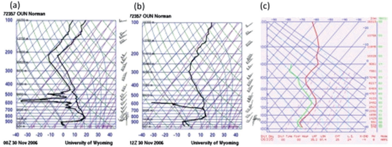
FIG. 3. Atmospheric soundings for Norman corresponding to the three precipitation types for the 30 Nov 2006 event from rawinsonde observations and RUC analysis at (a) 0000 UTC 30 Nov, (b) 1200 UTC on the same day, and (c) 0000 UTC 1 Dec (no radiosonde was launched at this time).
