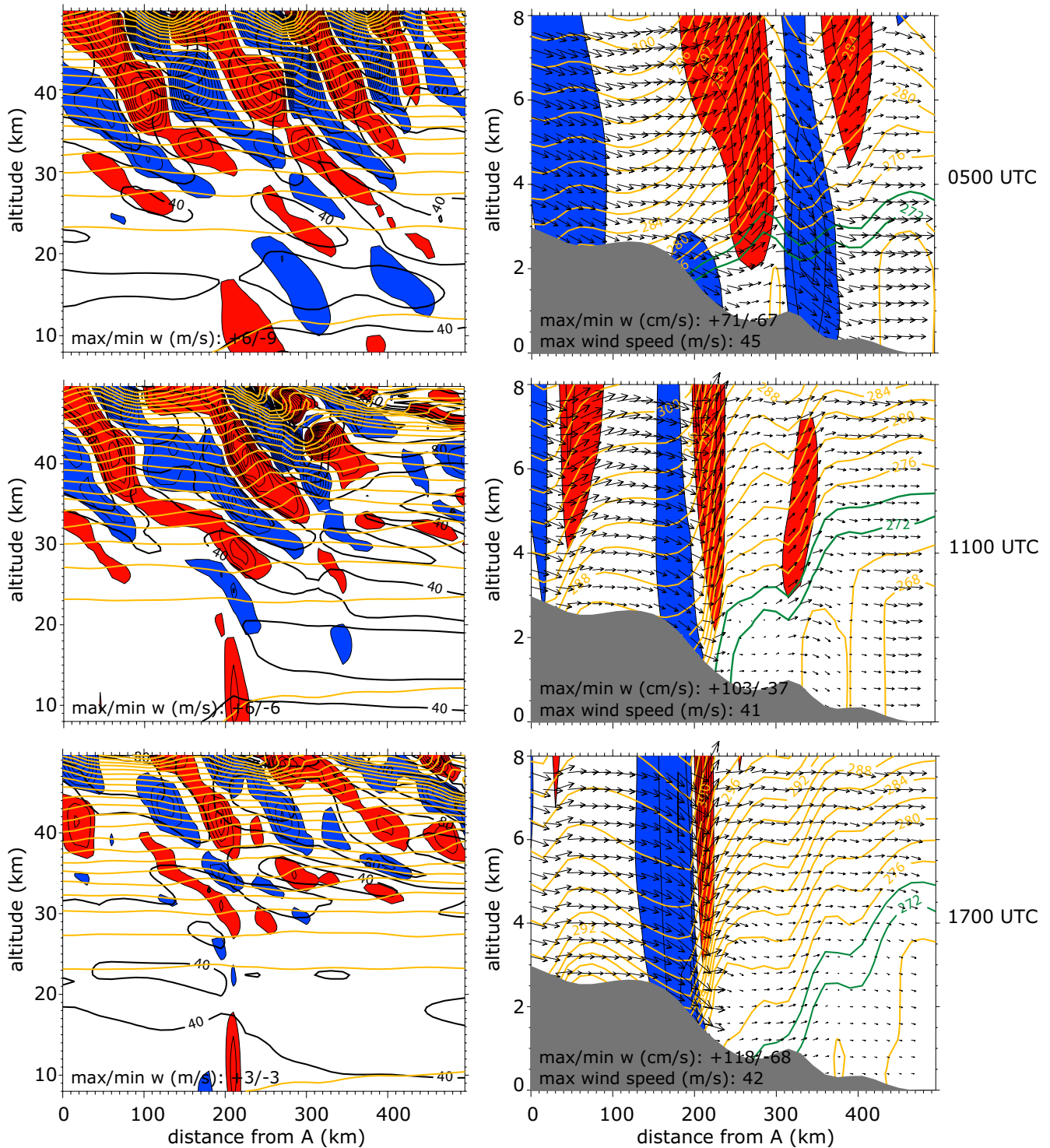
Figure 9. AB slice vertical cross-sections at every six hour of simulation. The left (right) diagram mainly covers the atmosphere above (below) 8 km. The vertical wind is shown as filled color contours (left: every 0.5 m/s; right: every 20 cm/s). The potential temperature is shown in orange contours (left: every 100 K; right: every 2 K). Green contours highlight the 272-274 K layer. The total horizontal wind speed is given as black contours (every 20 m/s) on the left panel. Cross-sectional wind is shown as vectors on the right. The Eastern Greenland terrain is shown in gray.
