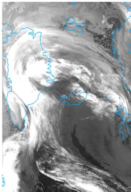
Figure 1. (a) AIRS observations (ascending orbits) at 2.5 hPa of radiance perturbations (of horizontal scales shorter than 500 km). (b) Infrared image from the Defense Meteorological Satellite Program (DMSP) at 0913 UTC 24 January 2005.
