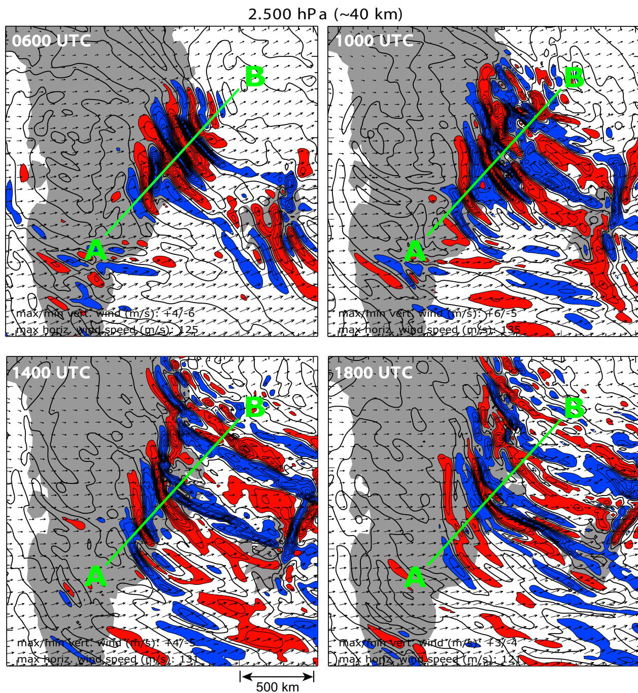
Figure 8. Evolution of the simulated 2.5-hPa vertical velocity every four hours in the rectangular region box shown in Fig. 7. Positive (negative) perturbation is shown in red (blue). Contour level is 0.5 m/s. The black contour indicates zero vertical velocity. Greenland and Iceland are shaded in gray. Vectors show the horizontal wind. Green line shows the AB slice used in subsequent figures.
