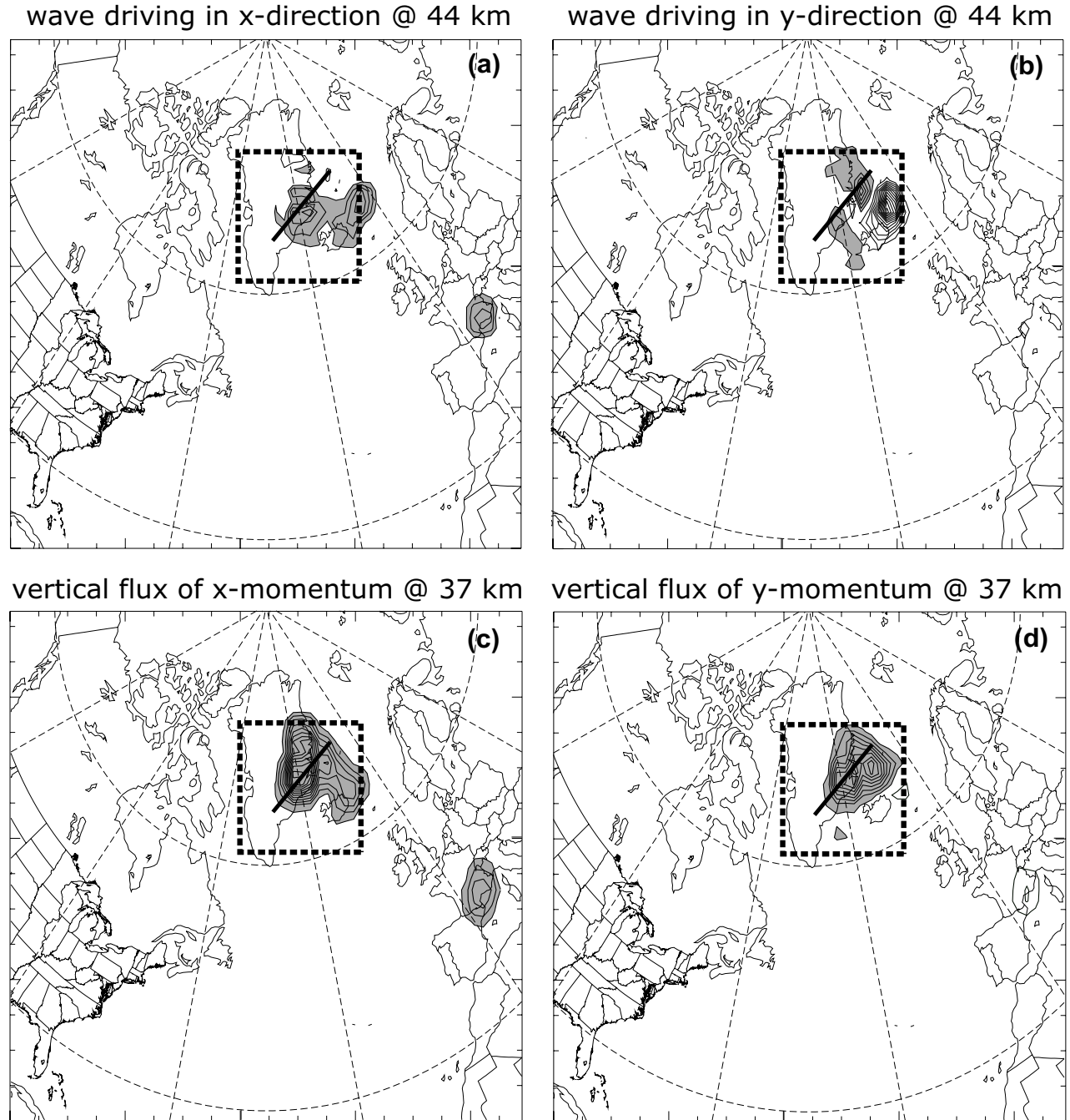
Figure 11. (a) Local wave driving in the x direction ( F_x , contoured every 0.1 \text{ m s}^{-1} \text{ hour}^{-1} ) at 44 km. (b) Same as (a) except in the y direction ( F_y ). (c) Vertical flux of momentum in the x direction contoured every 5 \times 10^{-3} \text{ kg m}^{-1} \text{ s}^{-2} at 37 km (d) Same as (c) except in the y direction. All negative contours are shaded. The thick line over Eastern Greenland indicates the AB slice and is shown for reference. The rectangular box indicates the region of focus shown in previous figures. All quantities shown are from the simulation at 1200 UTC.
