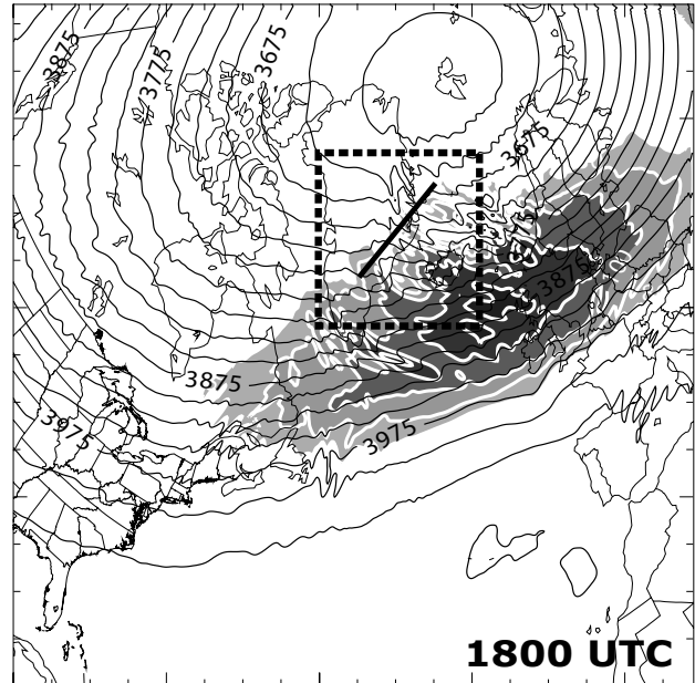
Figure 10. (Top row) GEOS-4 data at 0000 UTC (initial condition) and 1800 UTC of 24 January 2005. (Bottom row) ARPS simulation at 0600 UTC and 1800 UTC (initialized with 00 Z GEOS-4 data). The 2.5-hPa geopotential height is given in black contours (every 25 dam). Shaded regions show areas where the 2.5-hPa horizontal wind speed exceeds 80, 90, 100, 110, and 120 m/s (darkest). The thick line over Eastern Greenland indicates the AB slice and is shown for reference. The rectangular box indicates the region of focus shown in previous figures.
