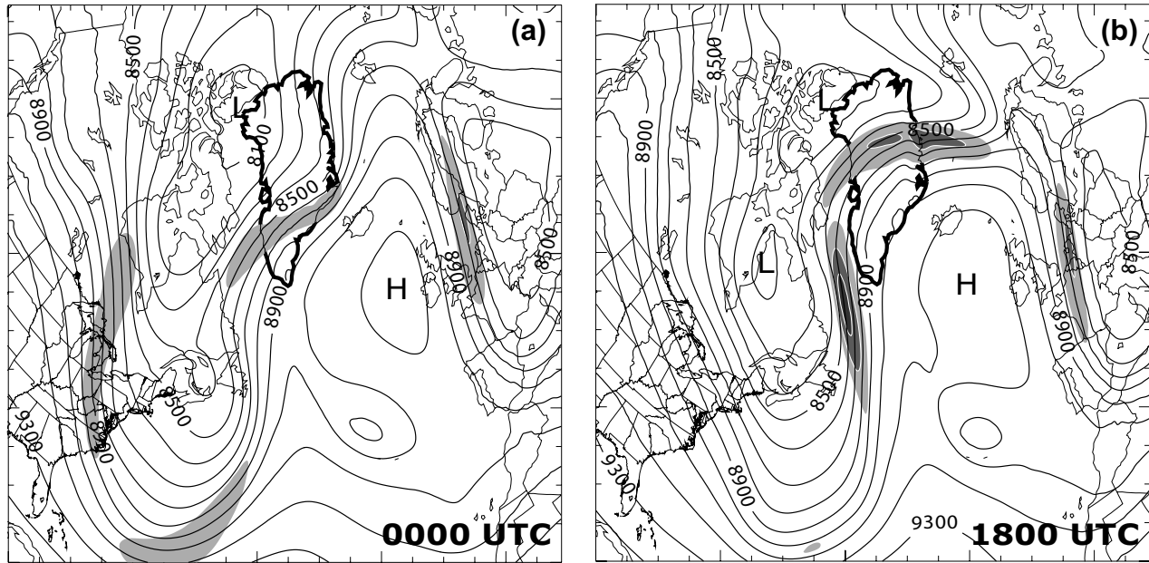
Figure 3. (a) GEOS-4 data at 0000 UTC of 24 January 2005 (initial condition). The 300-hPa geopotential height is given in black contours (every 100 m). Shaded regions show areas where the 300-hPa horizontal wind speed exceeds 60, 70, 80 m/s (darkest). (b) Same as (a) except at 1800 UTC. (c) Same as (a) except for the ARPS simulation at 1800 UTC (initialized with 0000 UTC GEOS-4 data). The 80-hPa vertical wind is given in filled color contours (every 0.1 m/s). Upward (downward) motion is shown in red (blue). Greenland is outlined in heavy black line.
