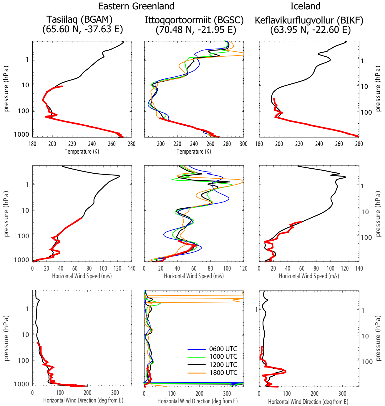
Figure 6. Soundings at Eastern Greenland (stations BGAM and BGSC) and Iceland (station BIKF) during 12 UTC 24 January 2005. The locations of these stations are shown in Fig. 5. Model (observational) data is shown in thick black (red) line. For BGSC, model profiles during other times are also shown.
