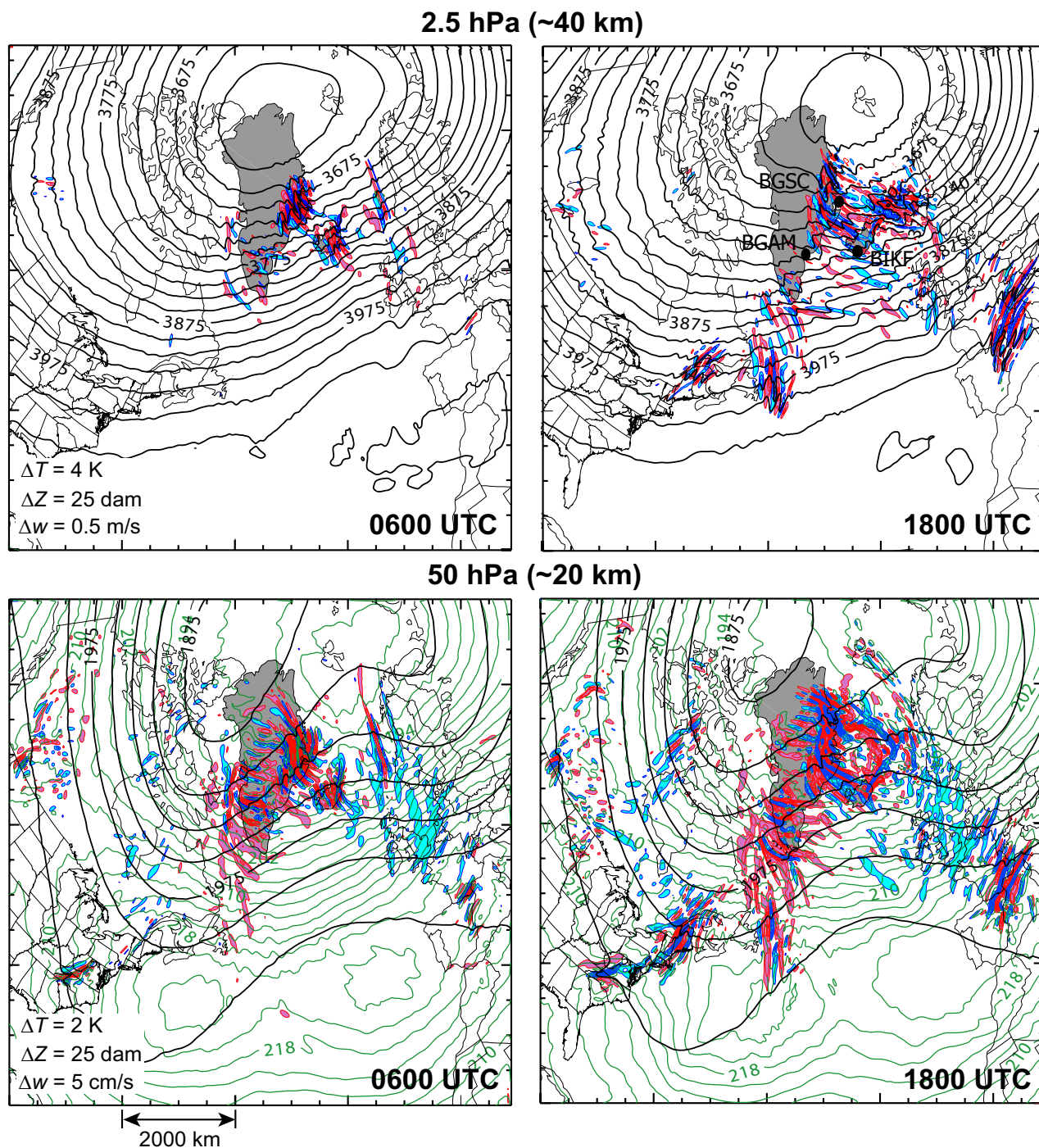
Figure 5. Same as Fig. 4 except at 2.5 and 50 hPa. Z is in decameter. For the 2.5-hPa diagram, the temperature contours are omitted for clarity. Black dots locate the observational stations at Tasiilaq (BGAM) and Ittoqqortoormiit (BGSC) on Eastern Greenland and at Keflavikurflugvollur (BIKF) on Iceland. Greenland and Iceland are shaded in gray.
