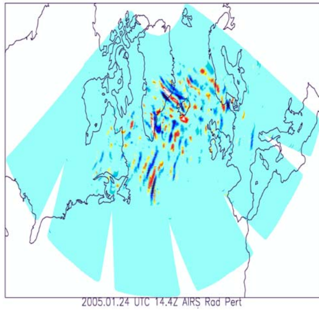
(a) AIRS Radiance Perturbation (< 500 km) 2.5 hPa, Color +/- 3.0K
