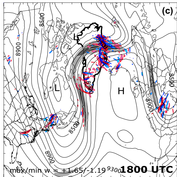
Figure 3. (a) GEOS-4 data at 0000 UTC of 24 January 2005 (initial condition). The 300-hPa geopotential height is given in black contours (every 100 m). Shaded regions show areas where the 300-hPa horizontal wind speed exceeds 60, 70, 80 m/s (darkest). (b) Same as (a) except at 1800 UTC. (c) Same as (a) except for the ARPS simulation at 1800 UTC (initialized with 0000 UTC GEOS-4 data). The 80-hPa vertical wind is given in filled color contours (every 0.1 m/s). Upward (downward) motion is shown in red (blue). Greenland is outlined in heavy black line.
