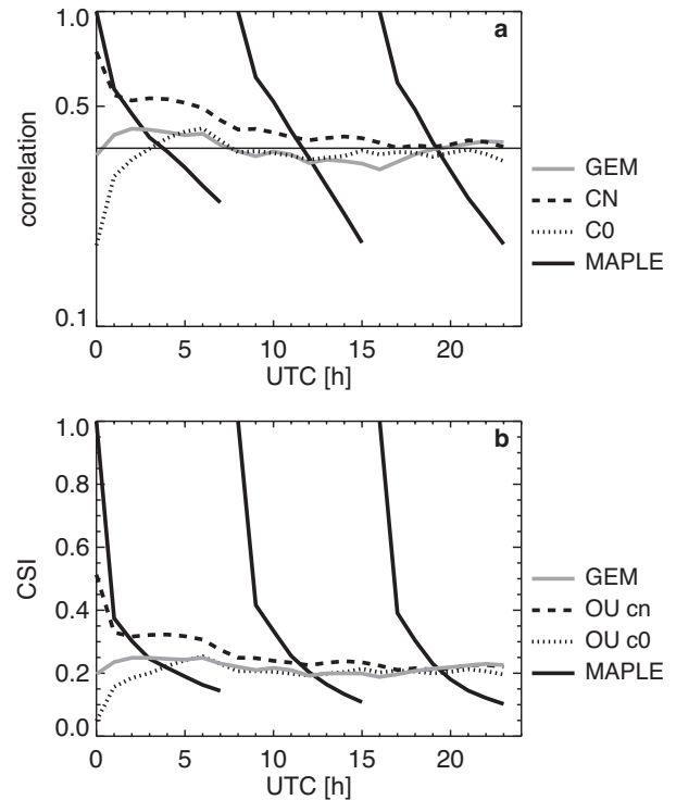
Fig. 5. Overall performance of the models as a function of time of the day. (a) correlation of the equivalent reflectivity fields (in dBZ); (b) Critical Success Index for the intensities over 0.2 mm/h.
