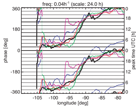
Fig. 4. Phase of the 24-hour harmonic as function of longitude corresponding to the average Hovmöller diagrams of Fig. 2 for rainfall accumulations. Different lines correspond to radar observations (thick black line), models (CN in green, C0 in magenta, GEM in red), and MAPLE (blue). The dotted lines indicate that the harmonic does not explain 10% of the observed variance.
