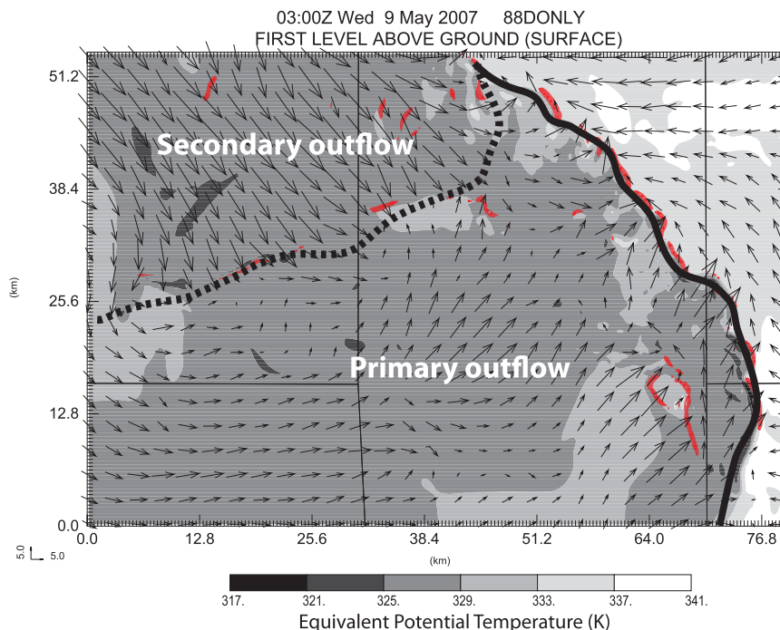
FIG. 12. As in Fig. 8, but for 88DONLY.
