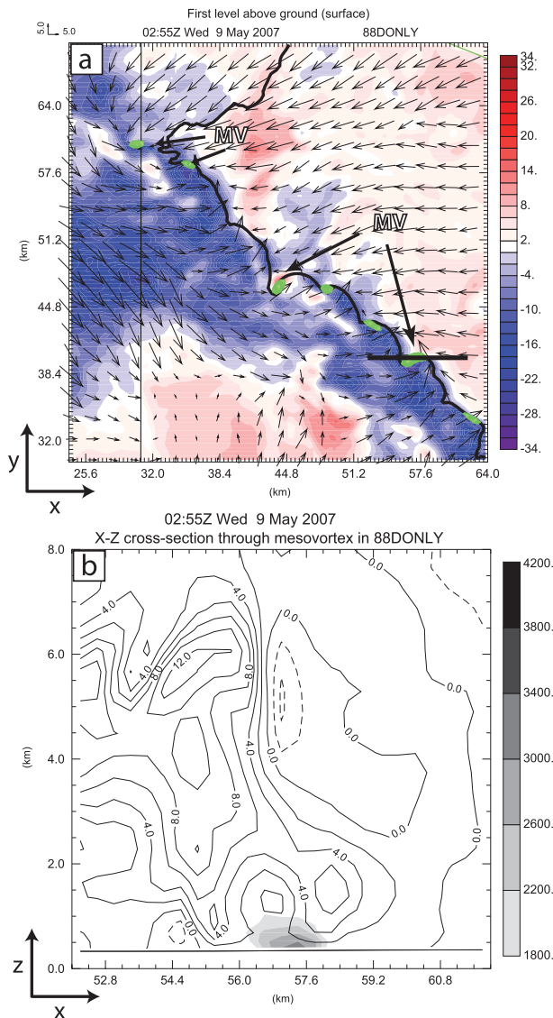
FIG. 13. (a) As in Fig. 9, but for 88DONLY at 0255 UTC and (b) x - z cross section along the thick black line in (a). “MV” marks vortices that meet the mesovortex criteria defined in the text. In (b) vertical velocity is contoured in 2 \text{ m s}^{-1} intervals and vertical vorticity is shaded at 400 \times 10^{-5} \text{ s}^{-1} intervals starting at 1800 \times 10^{-5} \text{ s}^{-1} .
