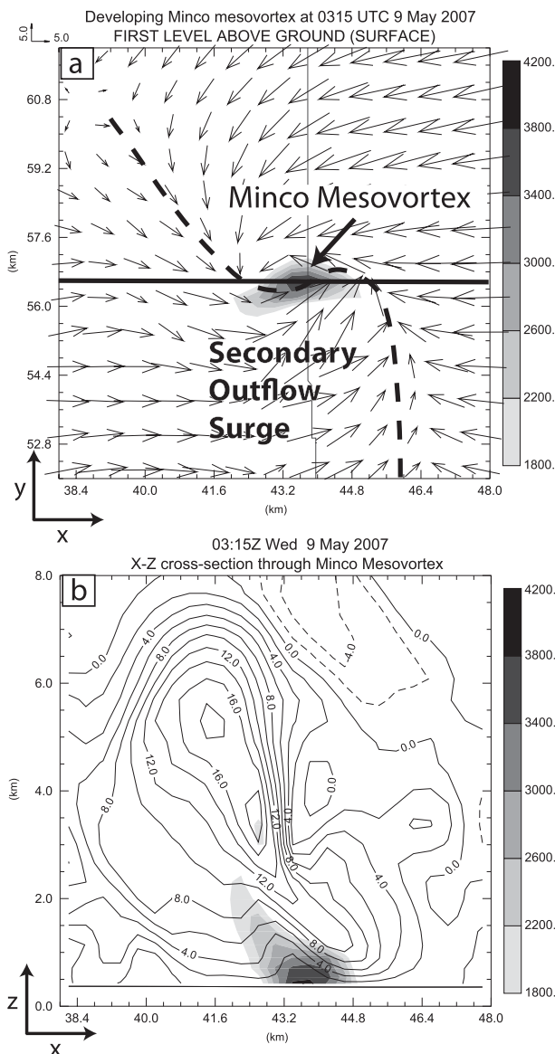
FIG. 10. (a) Horizontal wind and vorticity (shaded) at 0315 UTC 9 May 2007 from CASAvrZ and (b) x - z cross section through the developing Minco mesovortex along the thick black line in (a). The dashed line in (a) marks the locations of the secondary gust front. In (b) vertical velocity is contoured at 2 \text{ m s}^{-1} intervals. In both (a) and (b), vertical vorticity is shaded at 400 \times 10^{-5} \text{ s}^{-1} intervals starting at 1800 \times 10^{-5} \text{ s}^{-1} .
