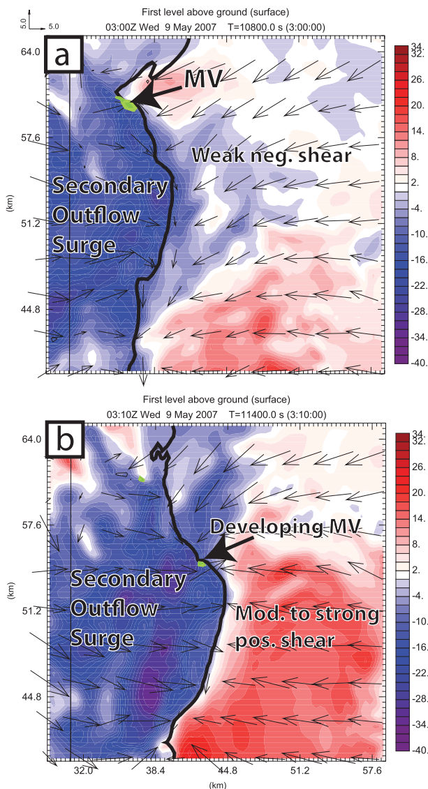
FIG. 9. Near-surface to 2.5 km AGL difference in magnitude of u -component velocity (shaded, \text{m s}^{-1} ) and near-surface velocity vectors ( \text{m s}^{-1} ) from CASAvrZ at (a) 0300 and (b) 0310 UTC. The small green shading areas are for vertical vorticity exceeding 1.4 \times 10^{-2} \text{ s}^{-1} . The thick black curve represents the 334-K equivalent potential temperature contour that marks the approximate location of the gust front. The MV denotes mesovortex.
