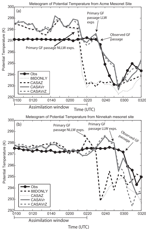
FIG. 4. Meteogram of potential temperature (K) observed and simulated at the (a) Acme and (b) Ninnekah mesonet sites from 0100–0320 UTC 9 May 2007. The gust front passage (GF) is noted for the NLLW and LLW experiments as well for the observations.
