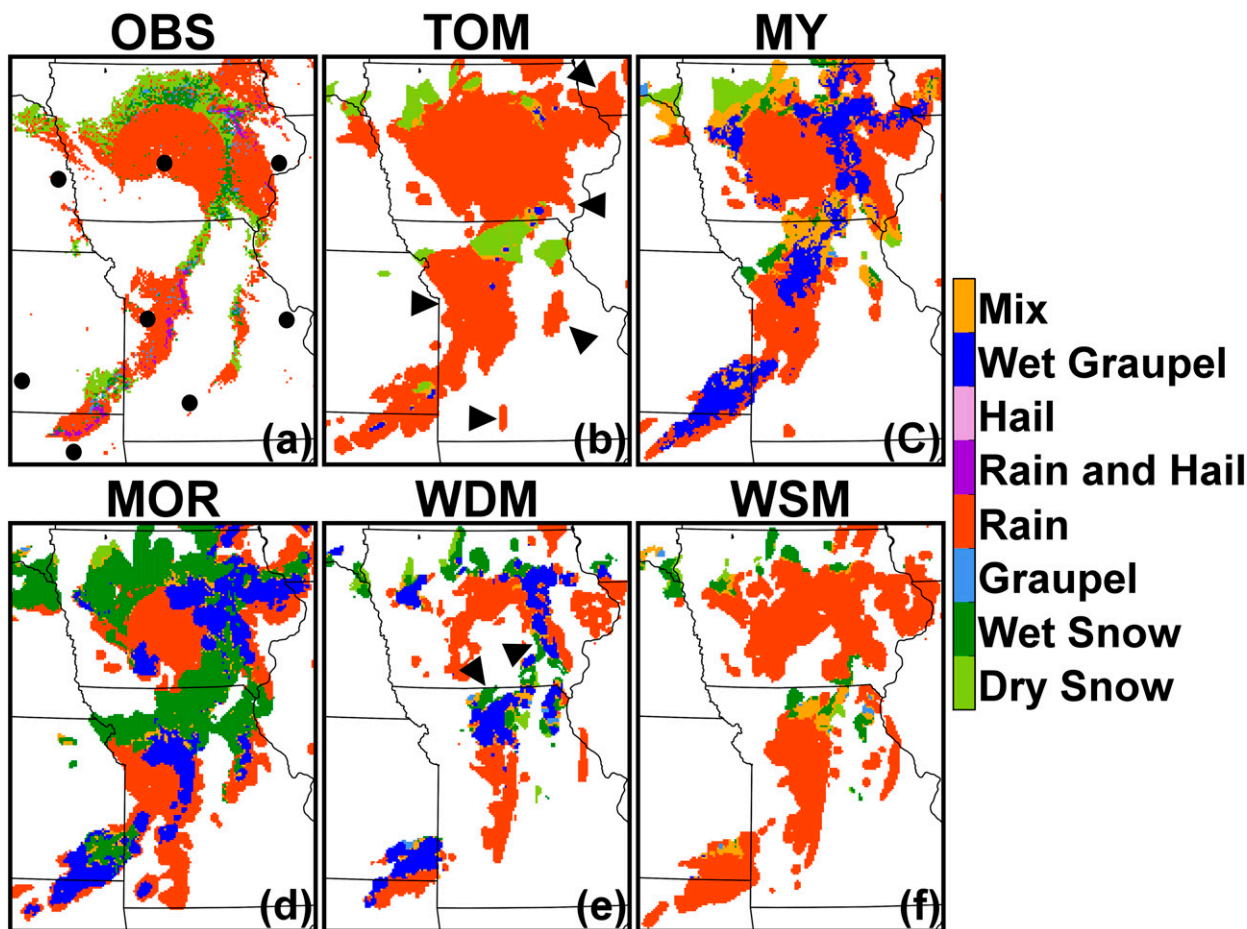
FIG. 6. Mosaic of hydrometeor classification using fuzzy logic for (a) observations at a 0.5^\circ tilt at 0400 UTC 20 May 2013 as well as classification of highest simulated linear reflectivity at the same tilt for the (b) TOM, (c) MY, (d) MOR, (e) WDM, and (f) WSM forecasts. Features of interest referenced in the text are noted by arrowheads. Locations of WSR-88D sites used for both the observed and simulated variable plots are noted with black dots in (a).
