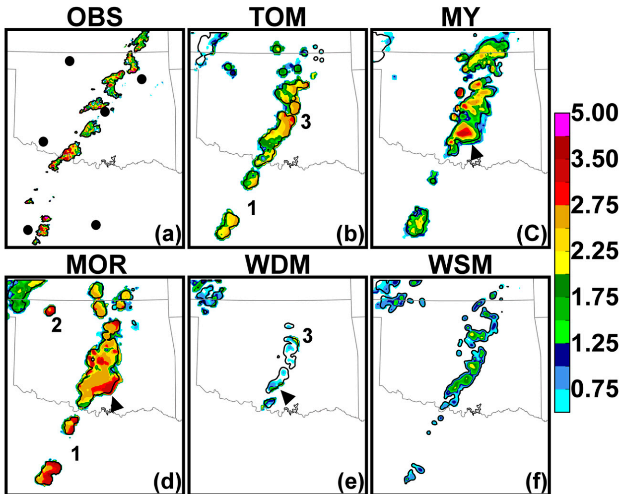
FIG. 12. As in Fig. 11, but for Z_{DR} (dB). Features of interest referenced in the text are noted by arrowheads and numbers.
