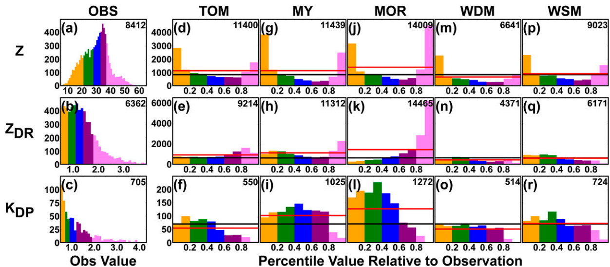
FIG. 7. Histograms of observed (a) reflectivity (dBZ), (b) differential reflectivity (dB), and (c) specific differential phase ( ^{\circ} \text{km}^{-1} ) mosaic values at a 0.5^{\circ} tilt from Figs. 3–5, as well as percentile histograms of simulated values at the same tilt from the (d)–(f) TOM, (g)–(i) MY, (j)–(l) MOR, (m)–(o) WDM, and (p)–(r) WSM forecasts distributed into bins based on the observed percentiles (noted by the horizontal solid black line). The idealized distribution given the number of values in each of the simulated results is indicated by the horizontal red line. The total number of values is noted in the top-right-hand corner of each panel. The observed values are used as the bounds for the percentile bins and are similarly color coded in both the observed and simulated value plots.
