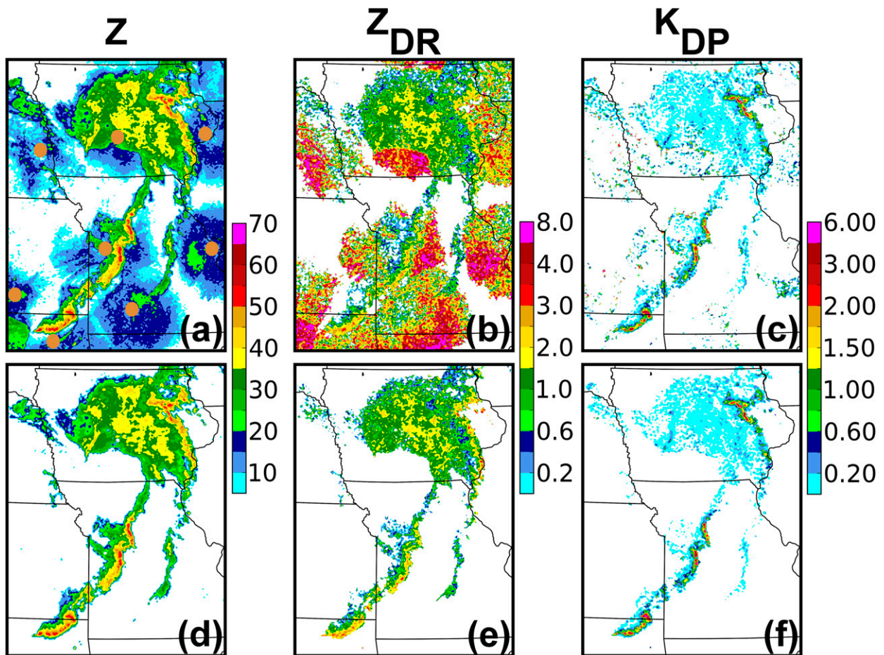
FIG. 2. Mosaics of observed (a) reflectivity (dBZ), (b) differential reflectivity (dB), and (c) specific differential phase ( ^{\circ} \text{ km}^{-1} ) at a 0.5^{\circ} tilt before ground clutter–biological scatterer removal and (d)–(f) after. The locations of the WSR-88D radars used are included as brown dots in (a).
