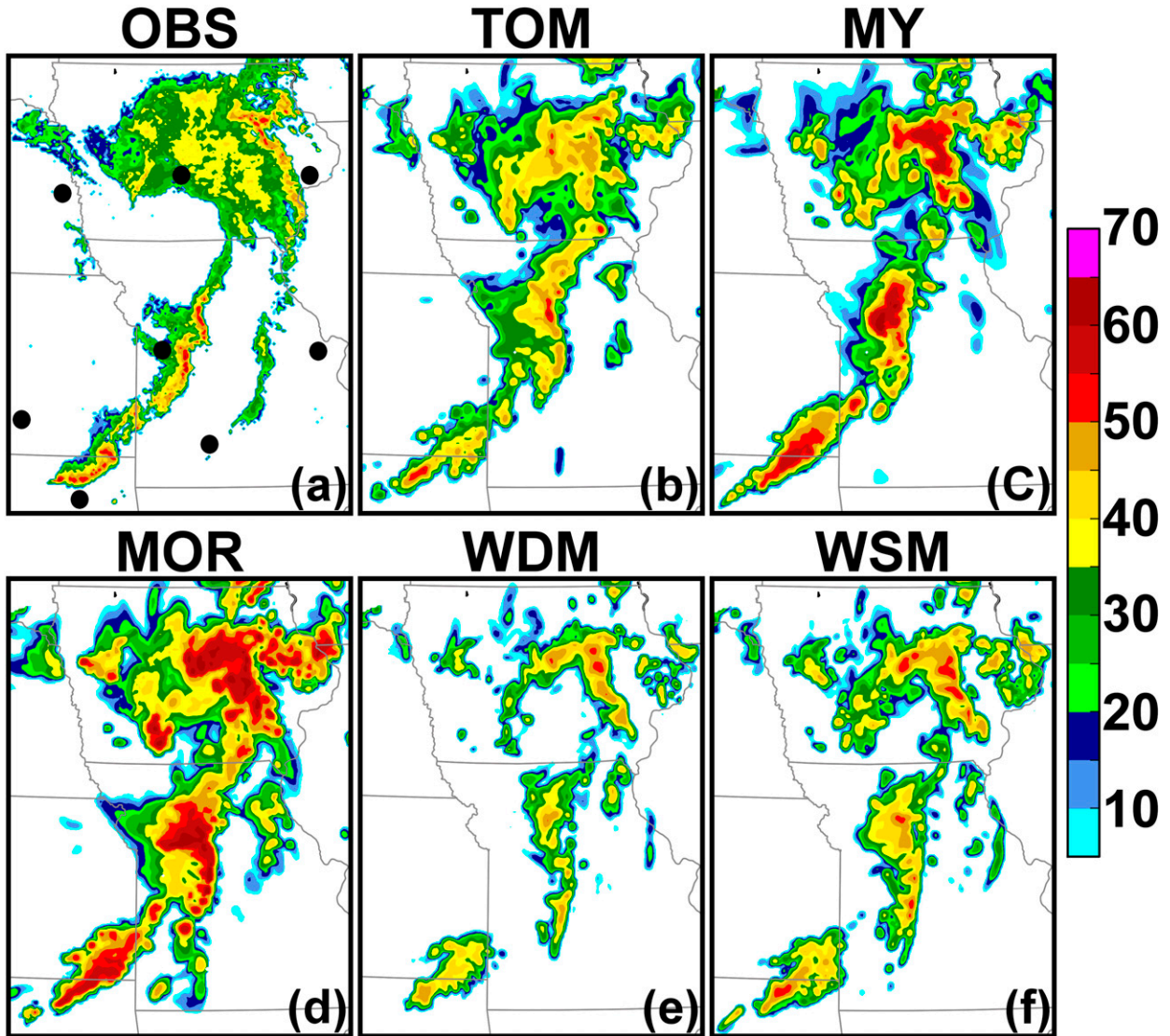
FIG. 3. Mosaics of observed (a) reflectivity (dBZ) at a 0.5^\circ tilt at 0400 UTC 20 May 2013 and simulated values at the same tilt from the (b) TOM, (c) MY, (d) MOR, (e) WDM, and (f) WSM forecasts. Locations of WSR-88D sites used for both the observed and simulated variable plots are noted with black dots in (a).
