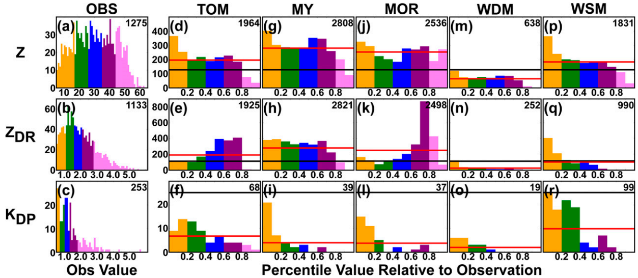
FIG. 16. As in Fig. 7, but from Figs. 11–13.
