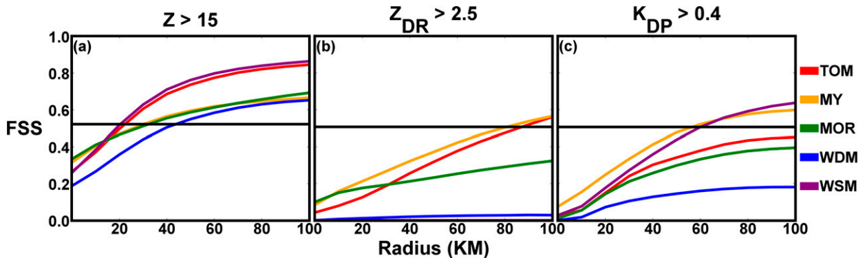
FIG. 17. FSSs for the TOM, MY, MOR, WDM, and WSM forecast results at increasing neighborhood radii for (a) reflectivity values > 15 \text{ dBZ} , (b) differential reflectivity values > 2.5 \text{ dB} , and (c) specific differential phase values > 0.4^\circ \text{ km}^{-1} for the mosaics in Figs. 11–13. The black line indicates skill greater than a random forecast.
