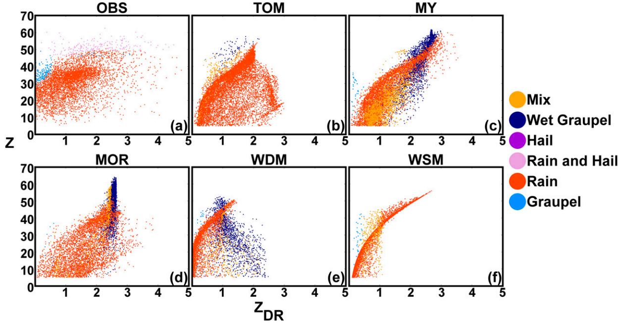
FIG. 8. Scatterplot of (a) observed reflectivity (dBZ) and differential reflectivity (dB) mosaic values at a 0.5^\circ tilt from Figs. 3–5, as well as scatterplots of simulated values at the same tilt from the (b) TOM, (c) MY, (d) MOR, (e) WDM, and (f) WSM forecasts.
