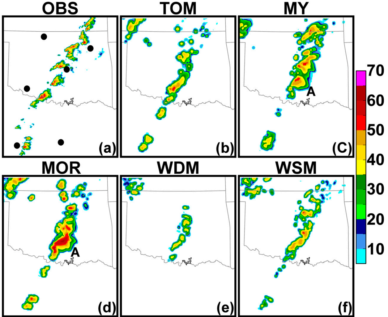
FIG. 11. Mosaics of observed (a) reflectivity (dBZ) at a 0.5^\circ tilt at 2100 UTC 20 May 2013 and simulated values at the same tilt for the (b) TOM, (c) MY, (d) MOR, (e) WDM, and (f) WSM forecasts. Features of interest referenced in the text are noted by capital letters. Locations of WSR-88D sites used for both the observed and simulated variable plots are noted with black dots in (a).
