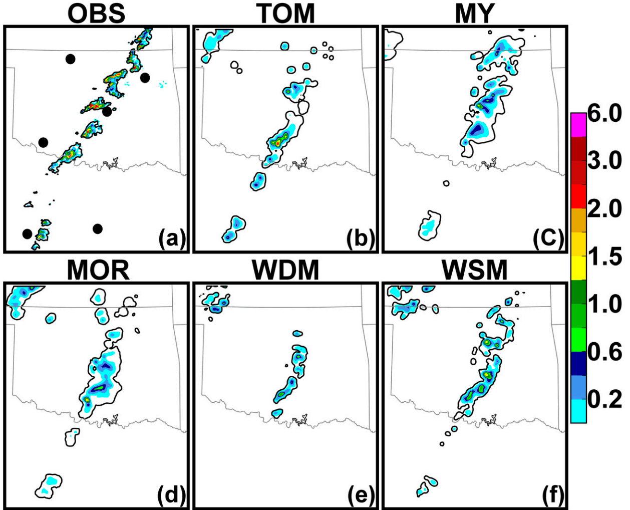
FIG. 13. As in Fig. 11, but for specific differential phase ( ^{\circ} \text{ km}^{-1} ).
