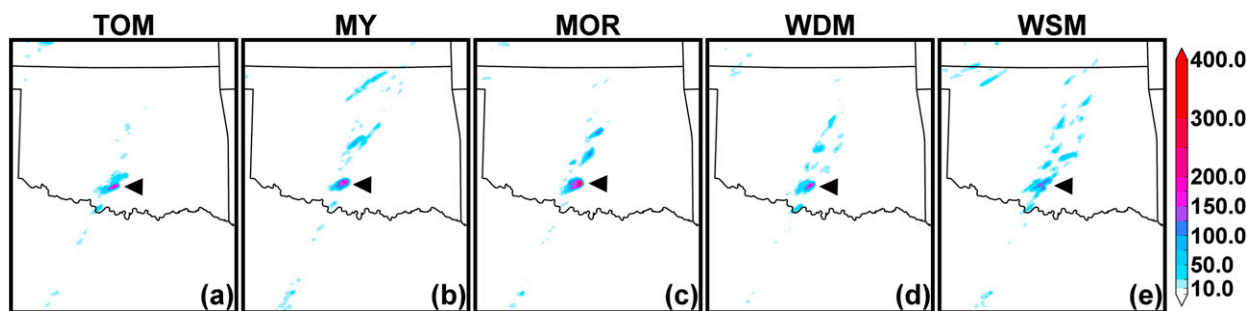
FIG. 15. 2D plots of maximum updraft helicity ( \text{m}^2 \text{s}^{-2} ) at 2100 UTC 20 May 2013 for the (a) TOM, (b) MY, (c) MOR, (d) WDM, and (e) WSM forecasts. Features of interest referenced in the text are noted by arrowheads.
