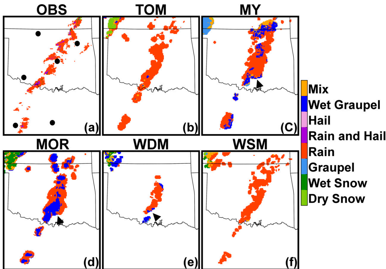
FIG. 14. Mosaic of hydrometeor classification using fuzzy logic for (a) observations at a 0.5^\circ tilt at 2100 UTC 20 May 2013, as well as classification of the highest simulated linear reflectivity at the same tilt for the (b) TOM, (c) MY, (d) MOR, (e) WDM, and (f) WSM forecasts. Features of interest referenced in the text are noted by arrowheads. Locations of WSR-88D sites used for both the observed and simulated variable plots are noted with black dots in (a).
