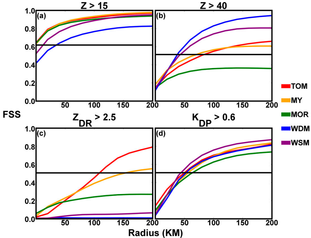
FIG. 9. FSSs for the TOM, MY, MOR, WDM, and WSM forecast results at increasing neighborhood radii for (a) reflectivity values > 15 dBZ, (b) reflectivity values > 40 dBZ, (c) differential reflectivity values > 2.5 dB, and (d) specific differential phase values > 0.6^{\circ} \text{ km}^{-1} for the mosaics in Figs. 3–5. The horizontal black line indicates skill greater than a random forecast.
