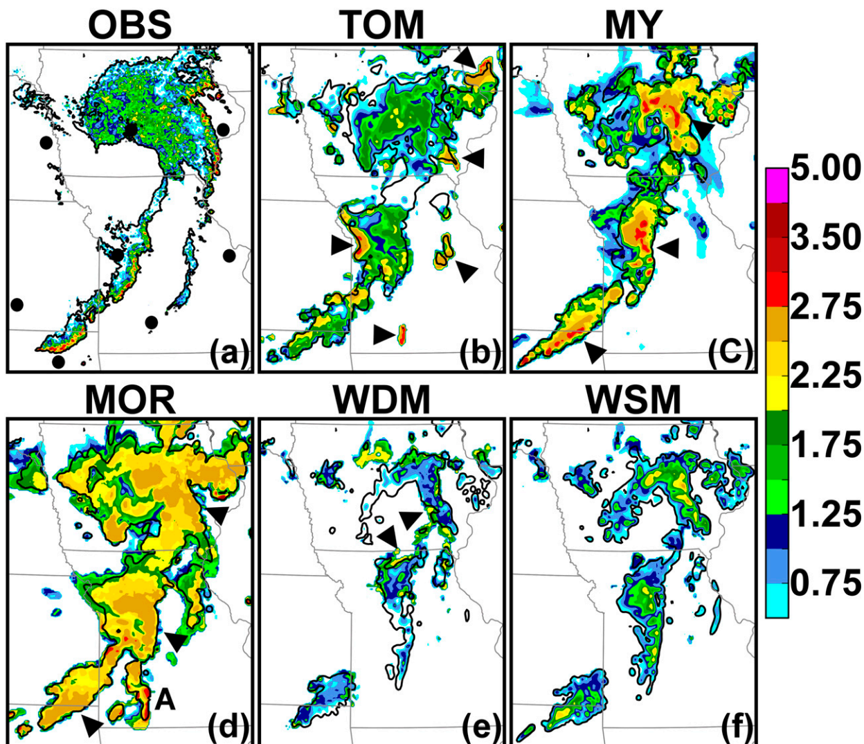
FIG. 4. As in Fig. 3, but for differential reflectivity (dB). Features of interest referenced in the text are noted by arrowheads.
