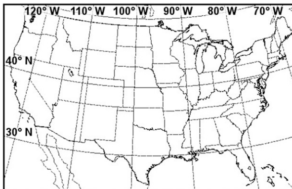
FIG. 1. Model domain for 2013 CAPS Spring Experiment SSEFs.
