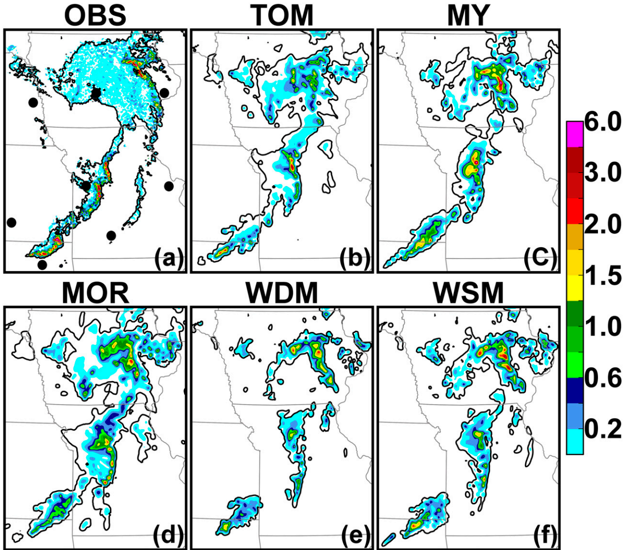
FIG. 5. As in Fig. 3, but for specific differential phase ( ^{\circ} \text{km}^{-1} ).
