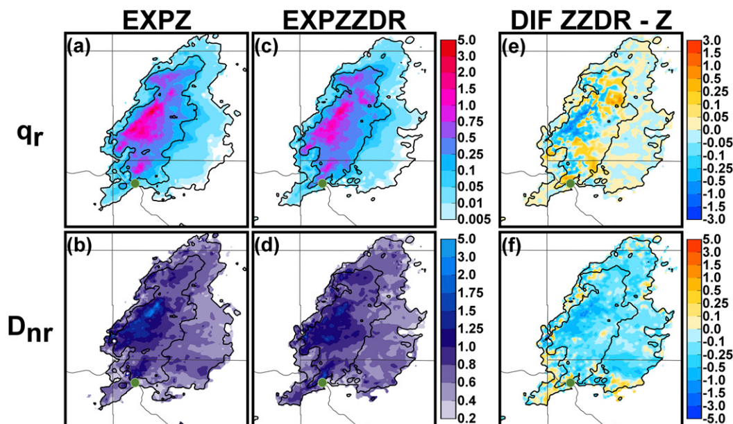
FIG. 13. (a) Rainwater mixing ratio ( \text{g kg}^{-1} ) and (b) mean mass diameter (mm) at 2 km AGL from the ensemble mean analyses at 1940 UTC for EXPZ and (c), (d) EXPZZDR as well as the (e), (f) difference between EXPZZDR and EXPZ for both fields. Reflectivity increments of 20 dBZ for EXPZ and EXPZZDR are contoured in black in the first two columns and for EXPZZDR in the rightmost column. The green dot marks the location of the updraft based on a local maximum in vertical velocity.
