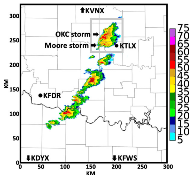
FIG. 1. 20 May 2013 experiment domain and location of radars assimilated. Observed reflectivity ( Z , dBZ) at the 0.5^\circ tilt from KTLX at 1938 UTC 20 May 2013 is included. The thin black line indicates the Oklahoma–Texas state boundary while the thin gray lines indicate county boundaries. The supercell associated with the Newcastle–Moore tornado is noted as the “Moore storm” and the supercell to the north discussed in the results is noted as the “OKC storm.” The evaluation domain used in section 4 is noted by the thick gray box.
