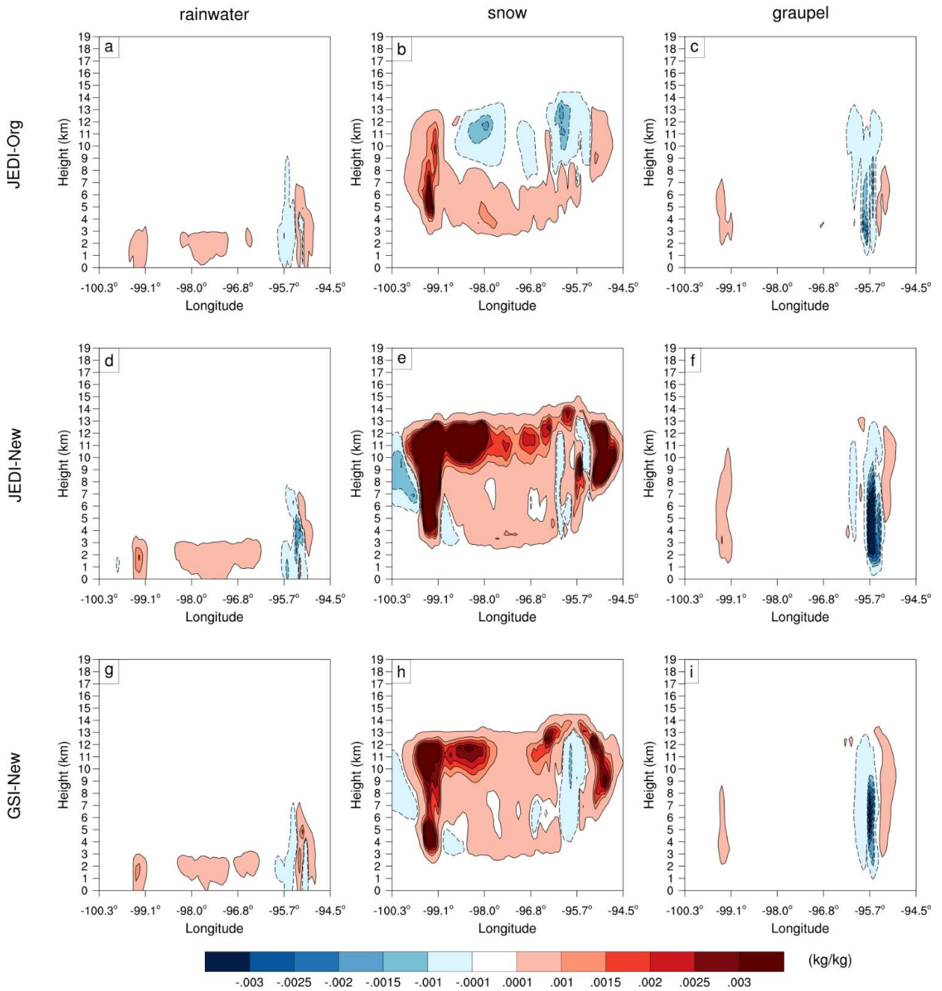
Figure 7. The vertical cross sections along the line given in Fig. 5 of analysis increments (kg kg -1 ) for hydrometeor mixing ratios of rainwater, snow, and graupel at final analysis time (00 UTC on May 13, 2022). The three columns correspond to rainwater, snow, and
