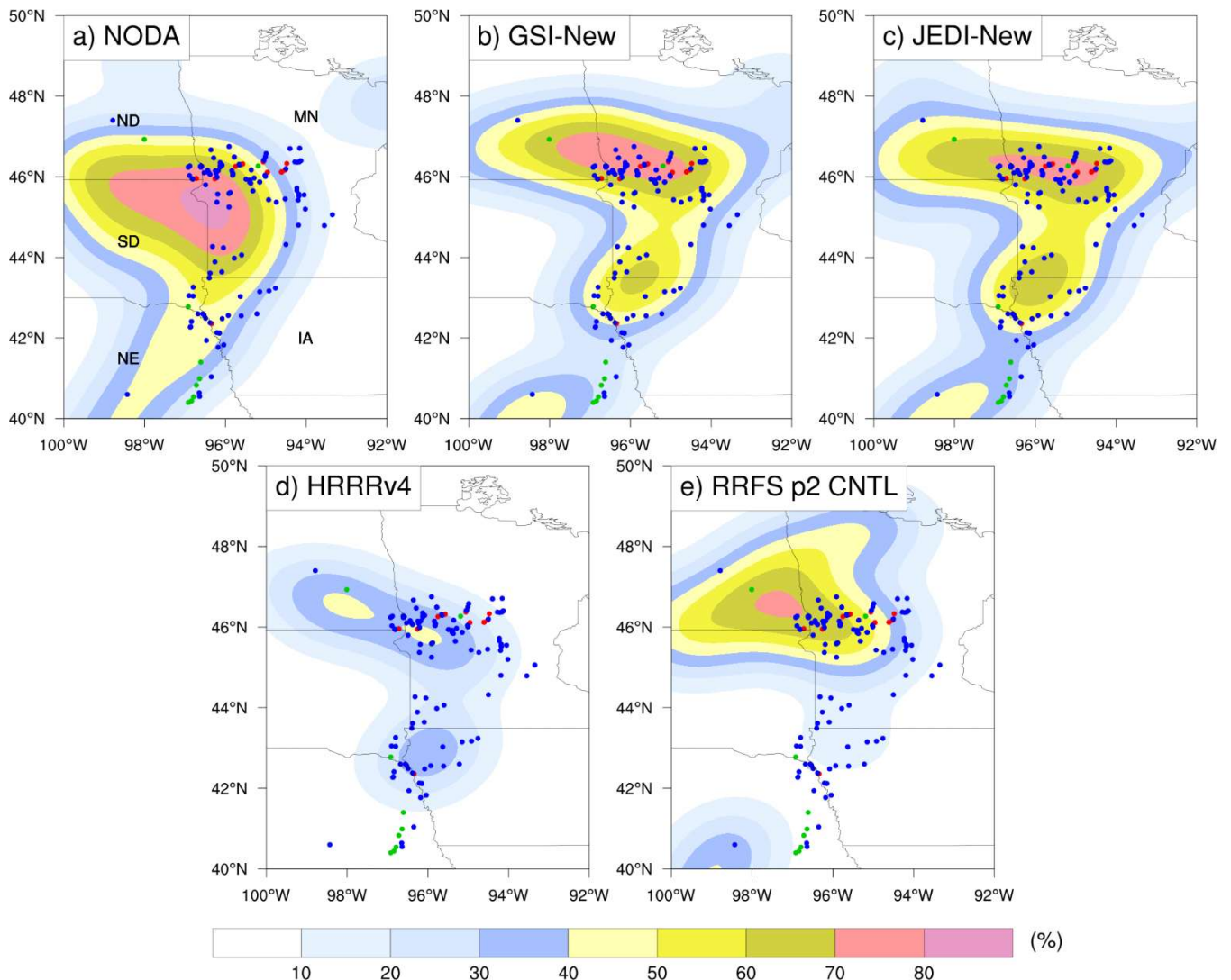
Figure 12. Neighborhood probability (%) (shaded) of 2-hr maximum updraft helicity exceeding 75 m 2 s -2 from 00 to 02 UTC on May 13, 2022 from the forecasts of a) NODA, b) GSI-New, c) JEDI-New, d) HRRRv4 and e) RRFS p2 CNTL. The red, green, and blue dots denote the SPC reports of tornado, hail, and wind, respectively.
