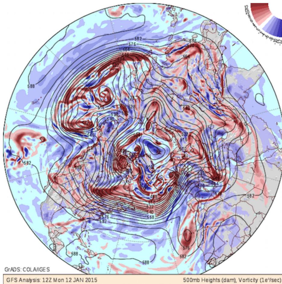
Figure 1: Hemispherical plot of 500mb height (contour) and vorticity (color) showing planetary scale waves.
