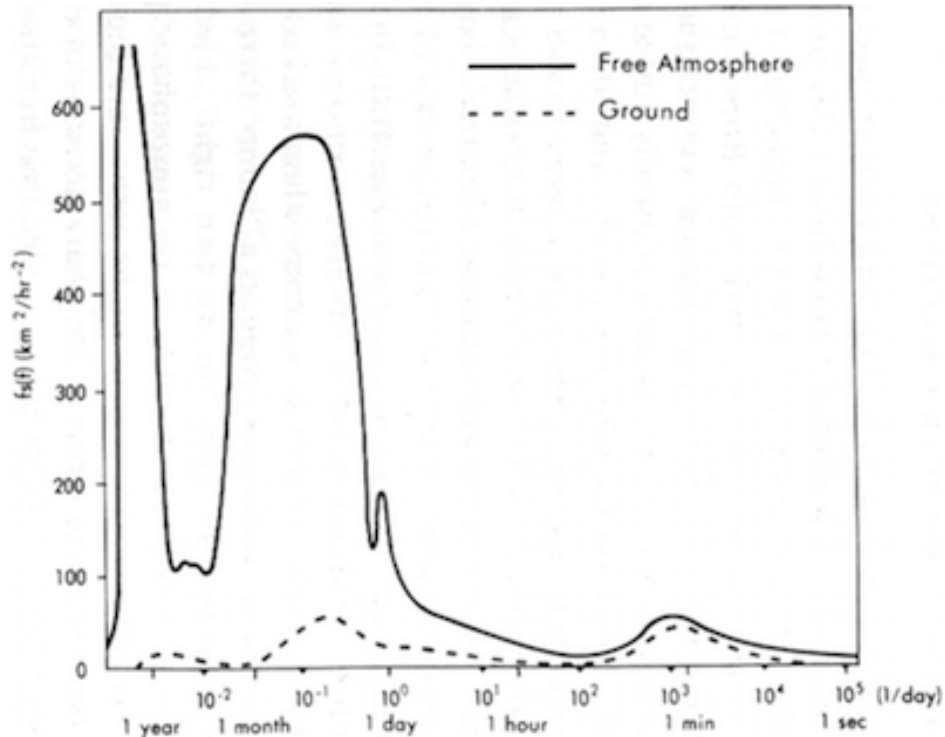
Figure 3: Average kinetic energy of west-east wind component in the free atmosphere (solid line) and near the ground (dashed line). (After Vinnichenko 1970 ; see also Atkinson 1981 )
