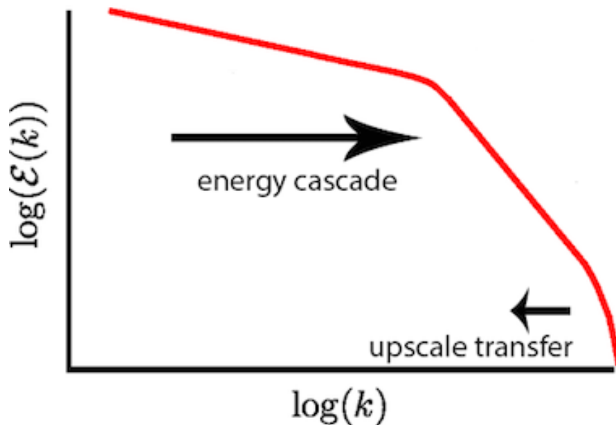
Figure 4: Depiction of the energy cascade. Here, E is energy and k is wavenumber.
