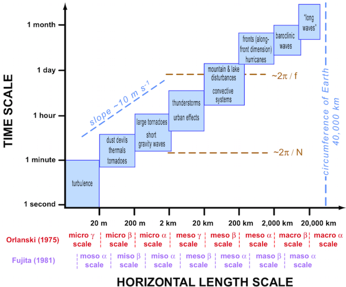
Figure 5: Scale definitions and the characteristic time and horizontal length scales of a variety of atmospheric phenomena. Classification schemes from Orlanski (1975) and Fujita (1981) also are indicated. [From Markowski and Richardson 2010 ]
