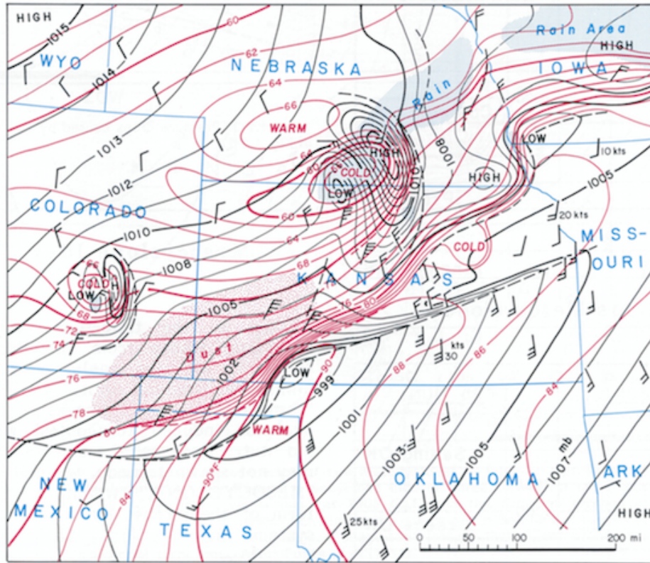
Figure 2: Sea level pressure (black contours) and temperature (red contours) analysis at 0200 CST 25 June 1953. A squall line was in progress at the time in northern Kansas, eastern Nebraska, and Iowa. [From Markowski and Richardson 2010 ]
