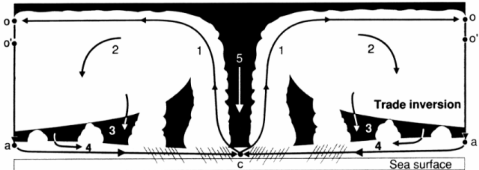
Fig. 9.14 Schematic cross section of the secondary meridional circulation in a mature hurricane. Air spirals in toward the eye (region 5) in the boundary layer (region 4), ascends along constant- M surfaces in the eyewall cloud (region 1), and slowly subsides and dries in regions 2 and 3. (After Emanuel, 1988.)
