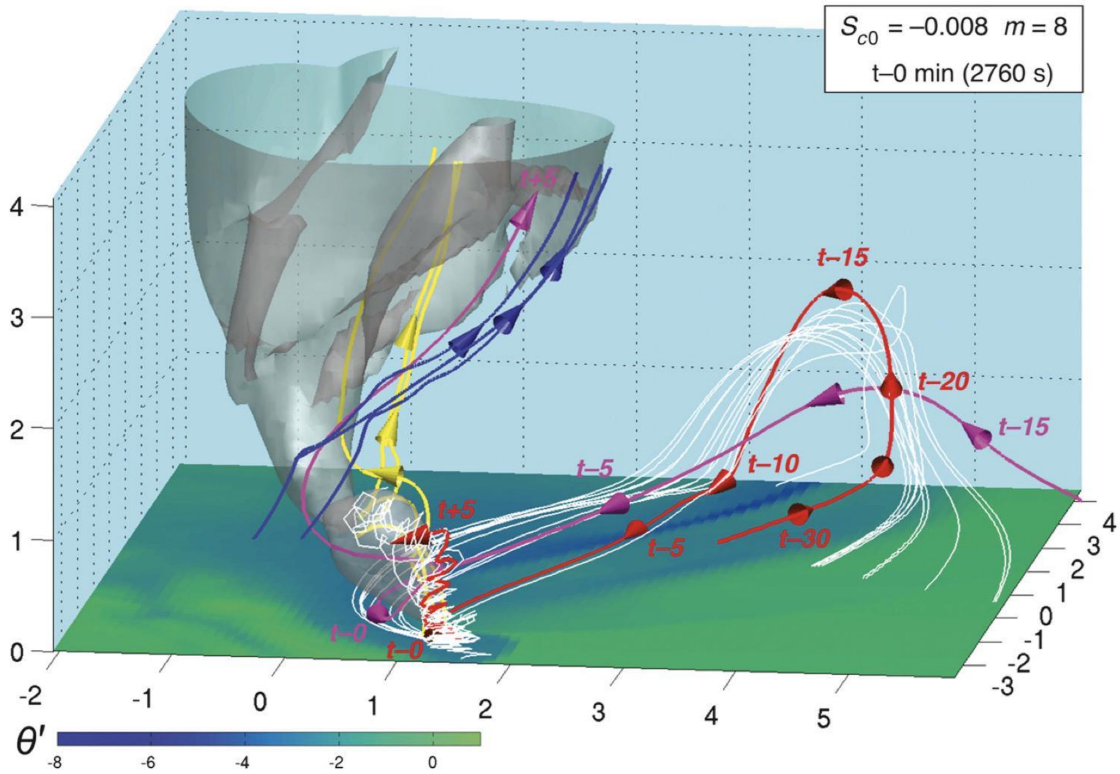
FIG. 8. As in Fig. 6, but at t - 0 min (2760 s) in the Sc8m8 simulation. The trajectories pass within 200 m of \zeta_{\max} , within 75 m of the surface, at t - 0 min. The trajectory that passes nearest to cyclonic vorticity maximum at t - 0 min is red. The magenta trajectory nears the lowest scalar level approximately 1 km west of \zeta_{\max} at t - 0 [see section 3a(3) and Fig. 11 for details]. The view is from the south-southeast.
