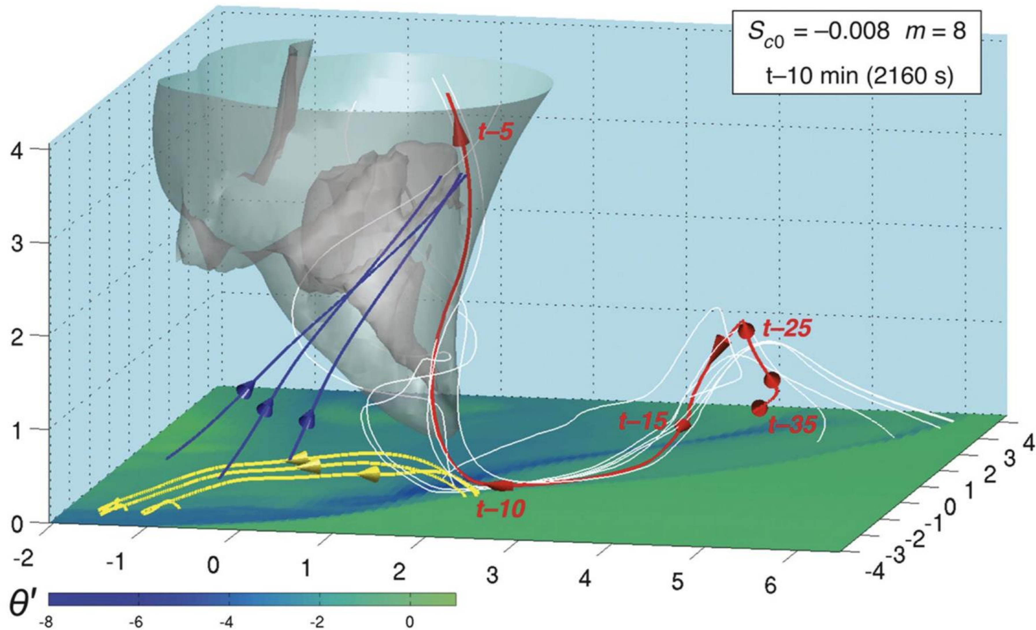
FIG. 6. Three-dimensional view of the midlevel updraft, near-surface \theta' field, and key vortex lines and trajectories at t - 10 min (2160 s) in the Sc8m8 simulation. The view is from the south-southeast. Axes are in kilometers. The w = 15 \text{ m s}^{-1} isosurface is gray. The near-surface \theta' field is color shaded (see legend). The yellow lines are vortex lines (their direction is indicated with arrows) that pass within 200 m of \zeta_{\max} at the lowest scalar level ( z = 50 m). The blue lines are vortex lines that pass within 500 m of \zeta_{\max} at z = 3 km. The white lines are forward-integrated trajectories that pass within 500 m of \zeta_{\max} at t - 10 min and have \zeta \geq 0.008 \text{ s}^{-1} in the lowest 75 m. The trajectory that passes nearest to the cyclonic vorticity maximum at t - 10 min is red. Arrows are placed along it at 5-min intervals.
