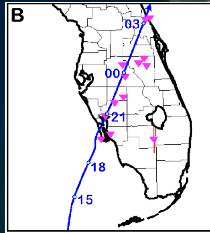
Buoyancy-Shear Overlap
