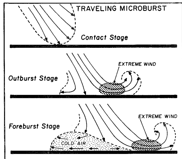
FIG. 28. Schematic diagram of a traveling microburst accompanied by an extreme wind near the ground.
