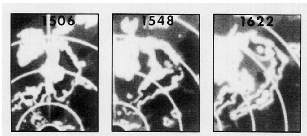
FIG. 25. Radar pictures showing a bow echo which turns into a spearhead echo and then into a comma echo. During its spearhead stage, this bow echo produced a cluster of 10 downbursts near Springfield, Illinois, on 6 August 1977 (25 n mi range markers). Refer to Fujita. 9
