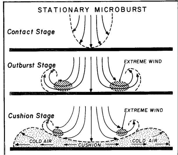
FIG. 27. Schematic diagram of a stationary microburst descending onto a cushion of cold air which weakens the outburst winds near the ground.
