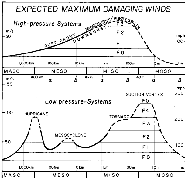
FIG. 32. Schematic distributions of expected maximum wind speeds induced by thunderstorms. The maximum winds associated with high-pressure systems are seen predominantly in misoscale outflow in microbursts and burst swaths. Maximum winds in low-pressure systems show several peaks of maximum winds corresponding to hurricanes, mesocyclones, tornadoes and suction vortices. Dashed curves denote unconfirmed wind speeds. Localized high winds beneath mesocyclones are often divergent, associated with twisting downburst.
