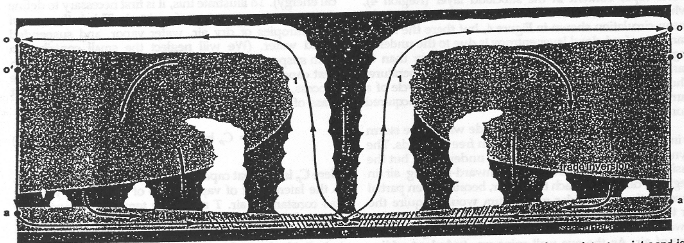
Figure 6. The structure and airflow of a mature hurricane are shown in this cross section, which spans a width of about 1,600 km and a height of 15 km. The regions correspond closely to those of the overall tropical atmosphere shown in Figure 4, but with an additional region of subsiding air in the eye (Region 5). In this case, the sea-surface temperature may be considered constant, but the total entropy content of the subcloud layer (Region 4) increases inward toward the eye as the increasing surface wind speed leads to greater evaporation rates, causing the near-surface air to approach
