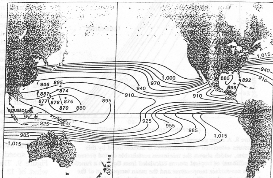
Figure 7. Hurricanes are areas of very low pressure. The tropical oceans are ideal spawning grounds for them, as demonstrated by this map, which shows the minimum sustainable central pressures in tropical storms under September mean climatological conditions over the Pacific Ocean and the Caribbean Sea. The pressures, which have been calculated using Eq. 5, are expressed in millibars, with 1,015 mb assumed to be the normal surface pressure. The dots and italicized numbers show, respectively, the locations and central pressures of some of the most intense hurricanes on record. Tropical storms in the Australian region are not indicated, because they occur during the late Southern Hemisphere summer (February–April).
