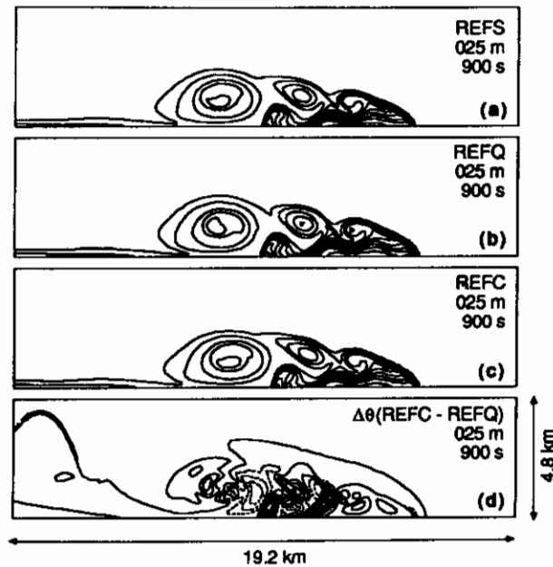
Figure 7. Plots of \theta' at 900 s for the 25.0 m solutions from the (a) staggered compressible reference model (REFS), (b) the quasi-compressible reference model (REFQ) and (c) the compressible reference model (REFC). The difference field of \theta' ( CI=0.5^\circ C ) between the 25.0 m solutions from the REFC and REFQ models is shown in (d) (as in Figure 1)
